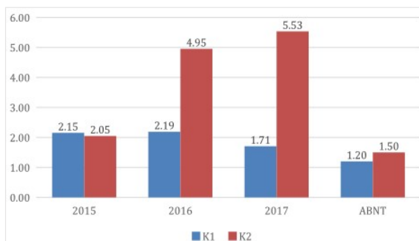
Figure 1 - Comparison between values calculated for the peak coefficients K_1 and K_2 and those suggested by the NBR 12218/2017 (Santos, 2018)
