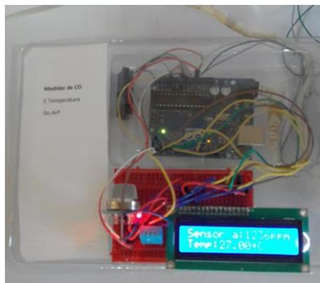
Figure 2 - System for measuring the production \text{CO}_2 in soil contaminated with soybean oil using the Arduino platform
