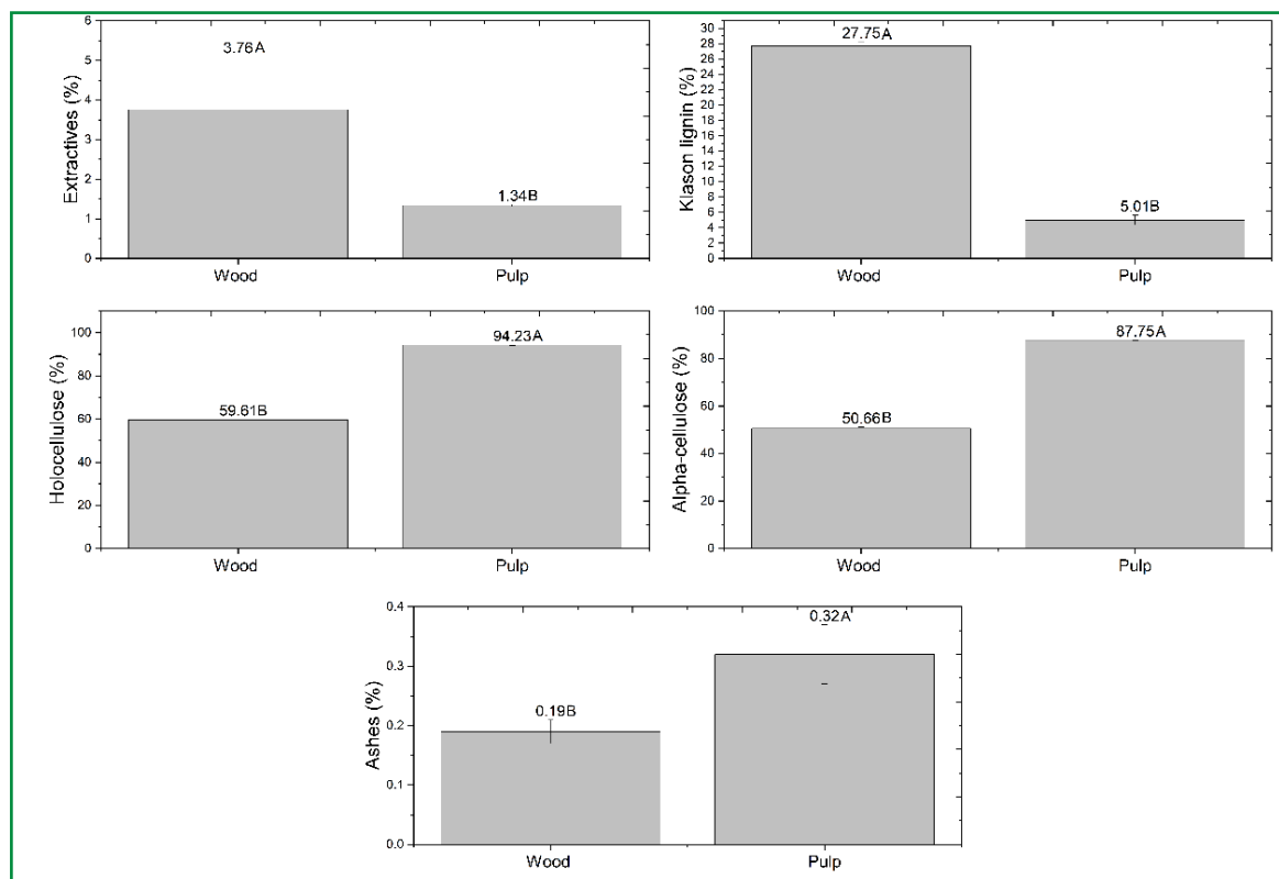
Figure 2 – Chemical composition of Pinus taeda wood and brown kraft pulp
