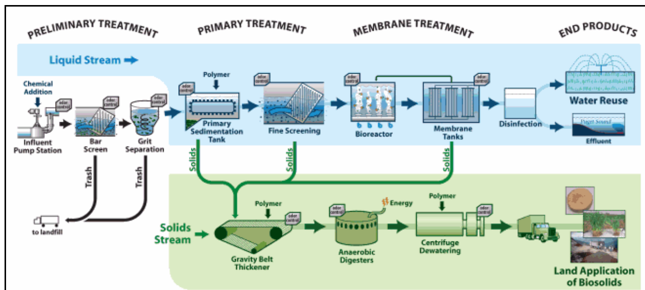
Figure 2 - Effluent Treatment Station
