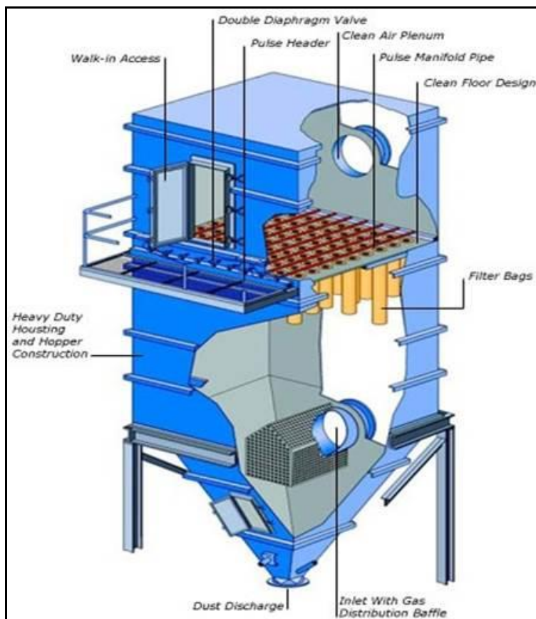
Figure 1 - Sleeve Filter
