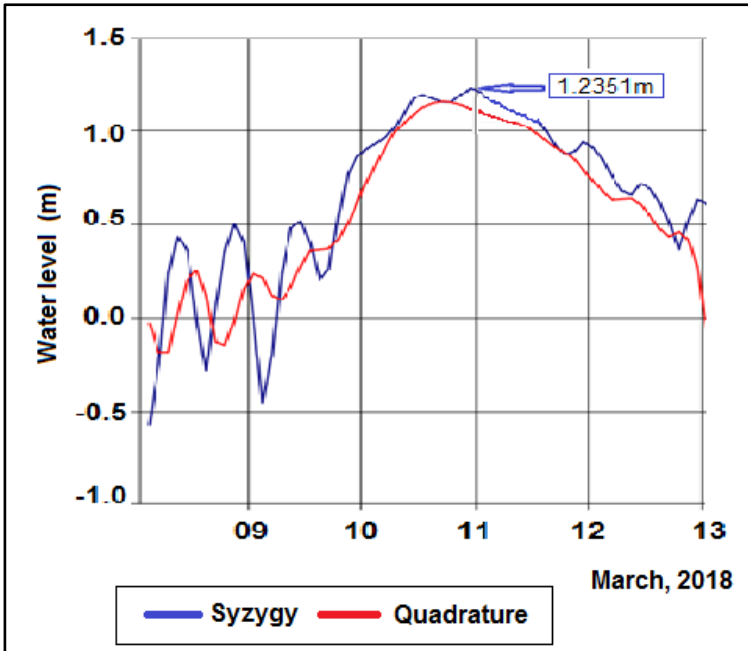
Figure 9 - Results of the water level in the Capote channel, with 10-years project rainfall
