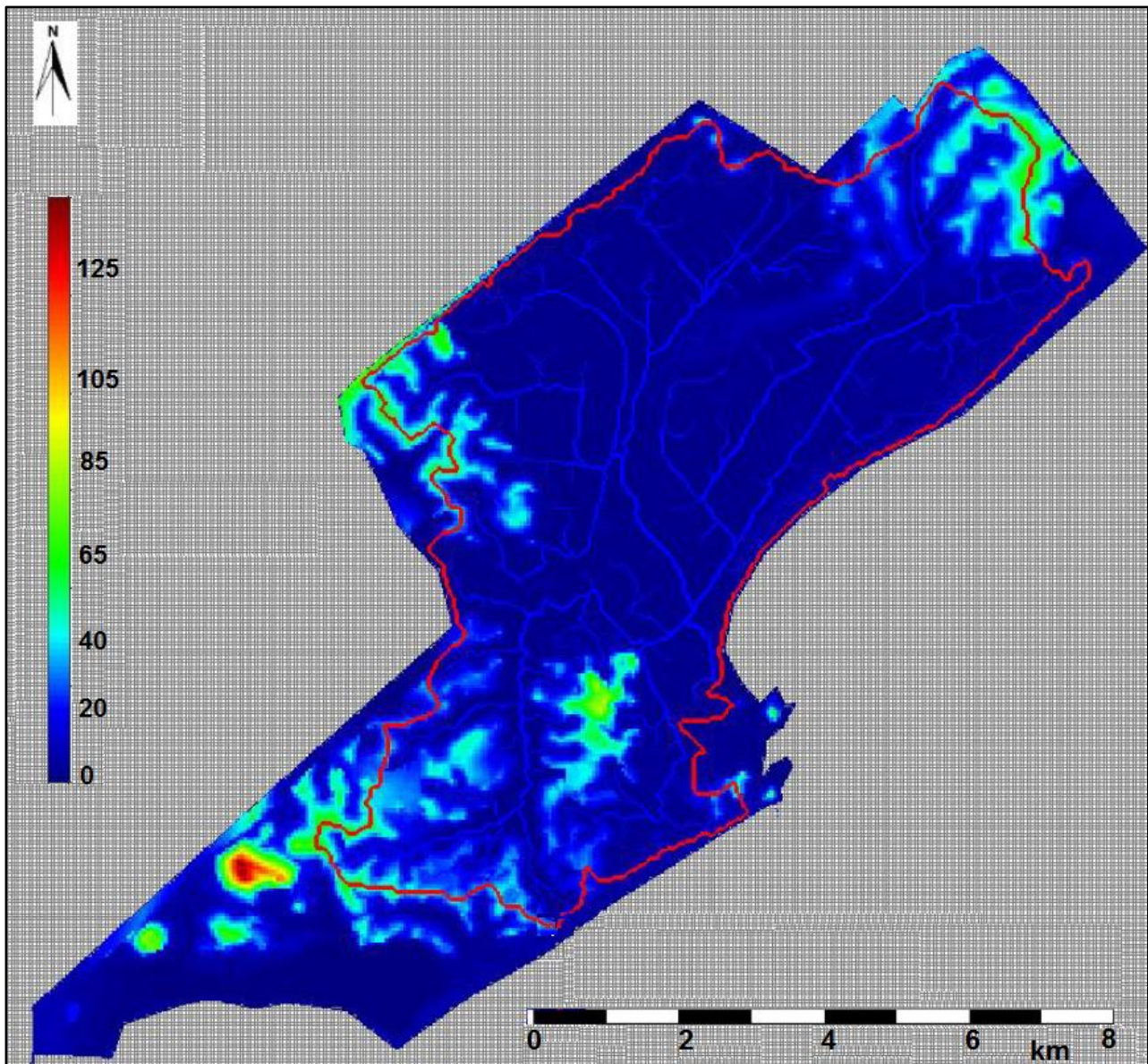
Figure 4 - Construction of Macaé DTM in MOHID GIS tool
