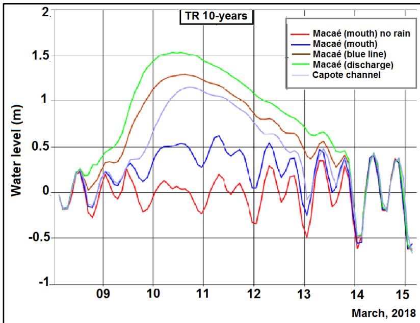
Figure 14 - Water level Simulation from the model of 10-years project rainfall and hydrographs of flow in the stations of Macaé river
