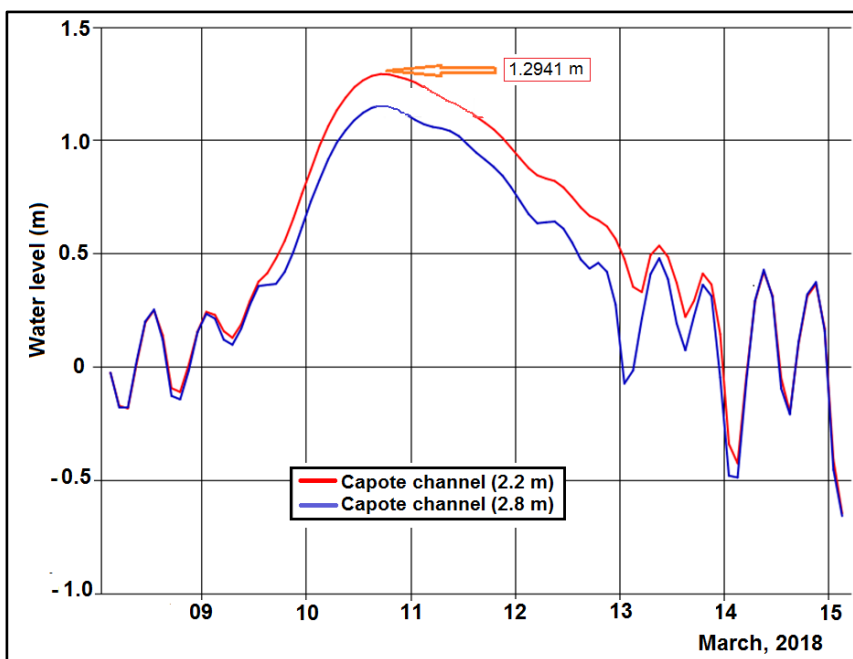
Figure 16 - Water level Simulation for Capote channel varying the depths of Macaé river (mouth)
