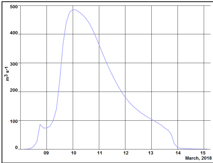
Figure 5 - Hydrograph for 10-years project rainfall in Macaé urban area for March, 2018
