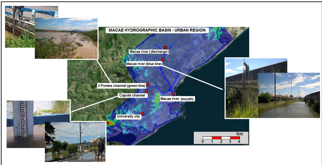
Figure 2 - In situ measurement positions at urban region of Macaé hydrographic basin
