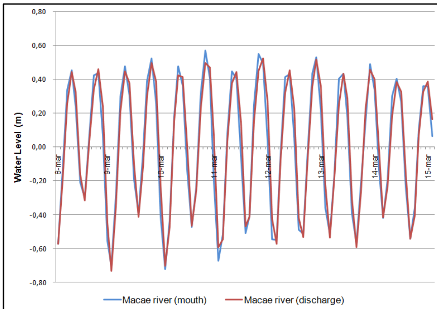
Figure 8 - Results of the water level in the sections of the Macaé river, with syzygy tide
