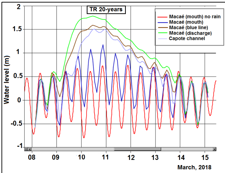
Figure 15 - Water level Simulation from the model of 20-years project rainfall and hydrographs of flow in the stations of Macaé river
