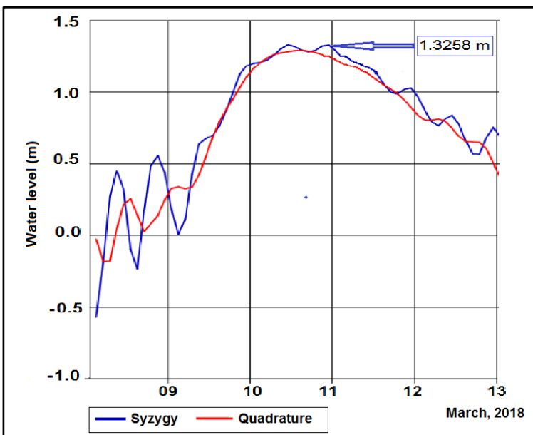
Figure 10 - Results of the water level in the Macaé river (Linha Azul), with 10-years project rainfall
