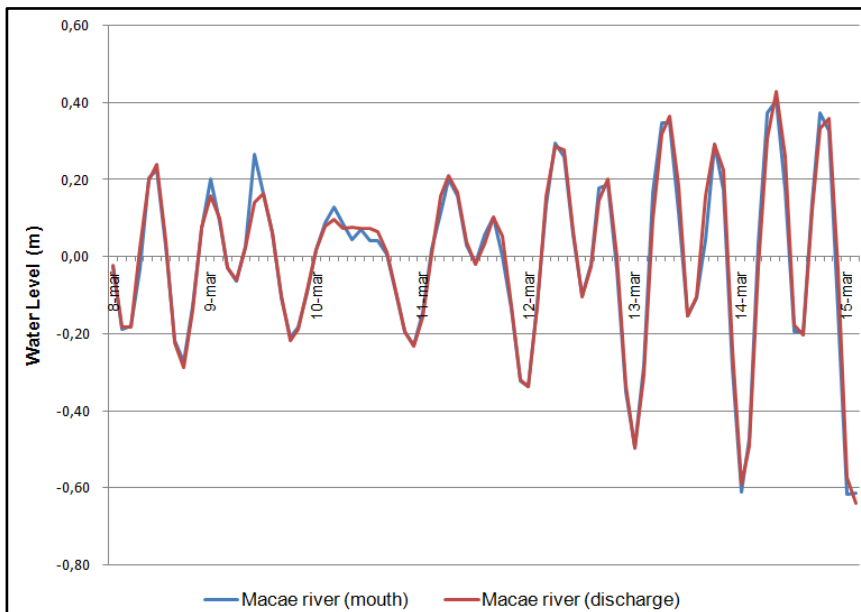
Figure 7 - Results of the water level in the sections of the Macaé river, with quadrature tide
