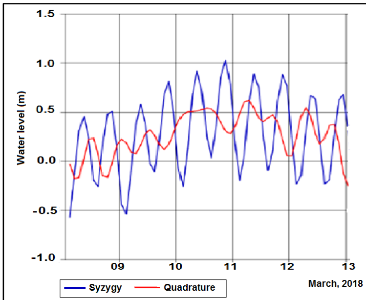
Figure 11 - Results of the water level in the Macae river (mouth), with 10-years project rainfall
