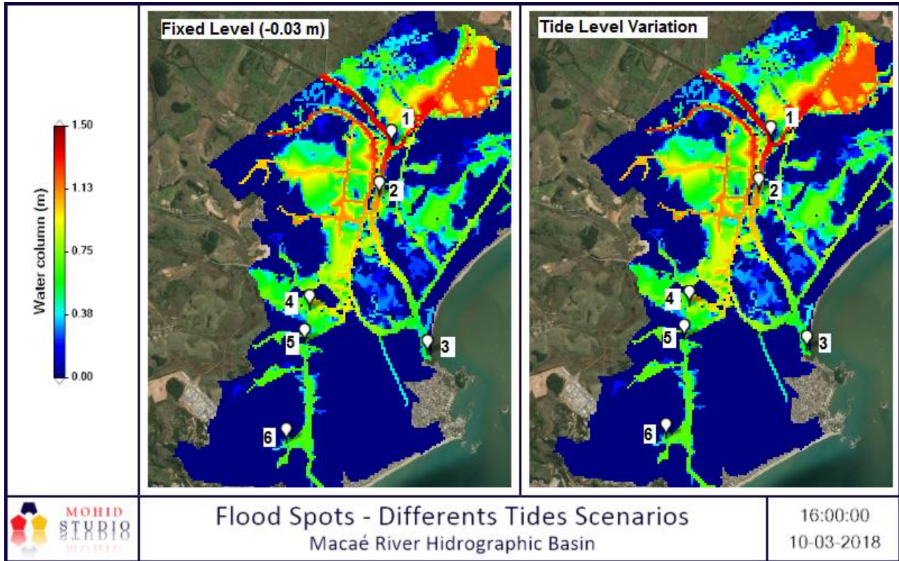
Figure 13 - Flood spots simulated to different tide level scenarios
