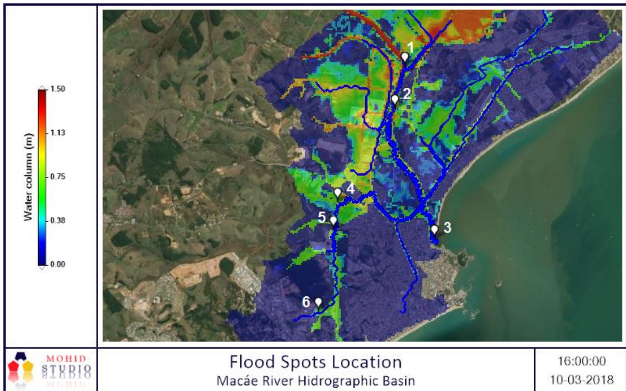
Figure 12 - Peak flood simulated to March, 2018 with 10-years rainfall project
