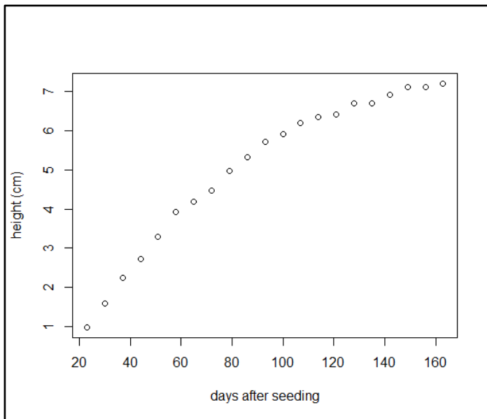
Figure 1 - Dispersion graph of the average height plant of the biquinho-type pepper as a function of time (days)
