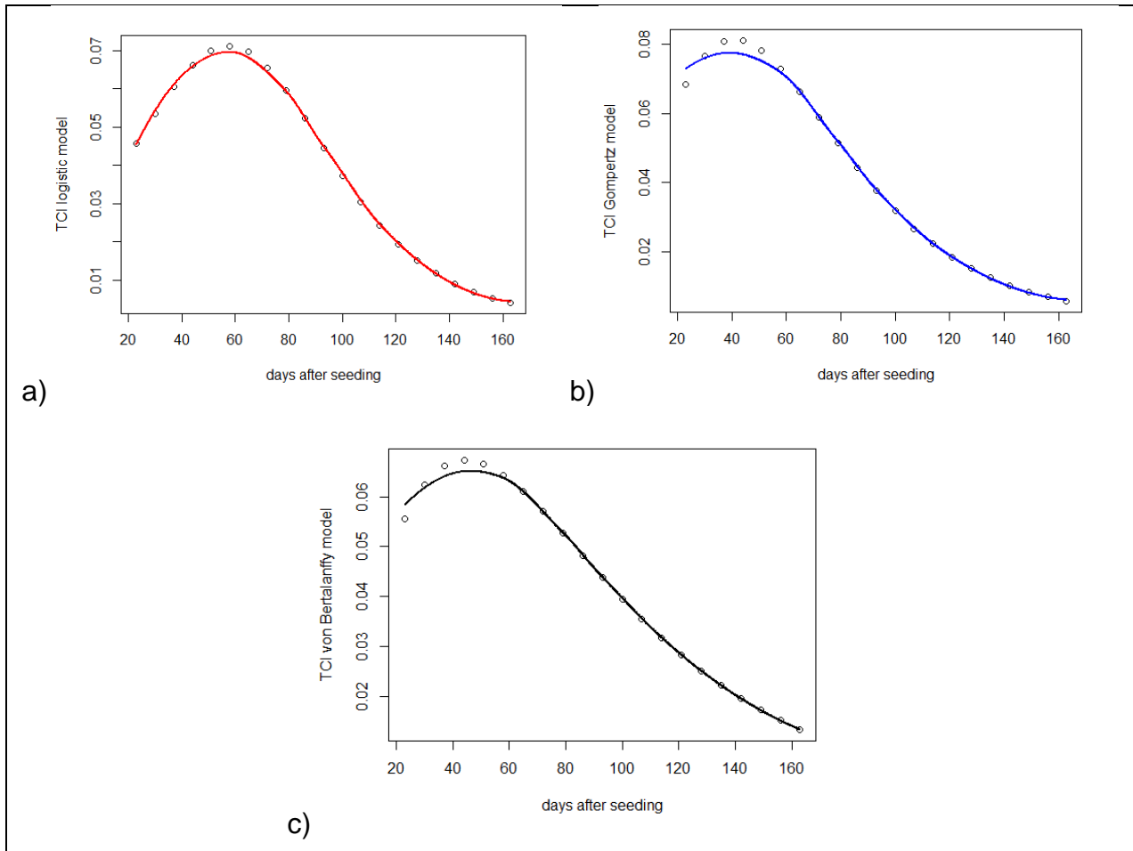
Figure 3 - Graphs of instantaneous absolute growth rates (TCI) for the logistic (a), Gompertz (b) and von Bertalanffy (c) models
