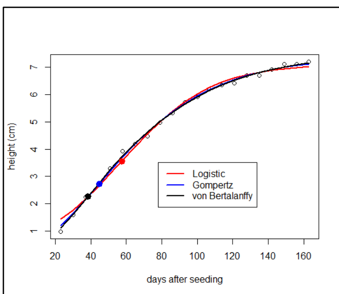
Figure 2 - Dispersion graph of the average height of the plant (cm) as a function of time (days) with the curves of the fitted models and the inflection points estimated with each adjustment
