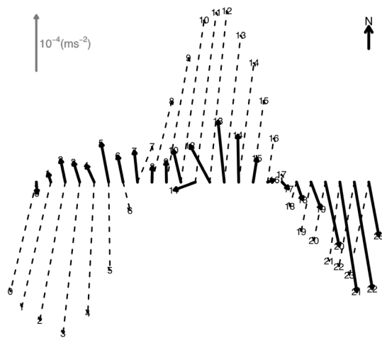
Figure 6: Near surface total wind vector tendency (solid arrows) and surface pressure-gradient-force (dashed arrows) for Chapadinha site. The number indicate the hour (GMT). This the gradient was obtained using the network of weather station from the INMET for the period between the years 2008 and 2012.
