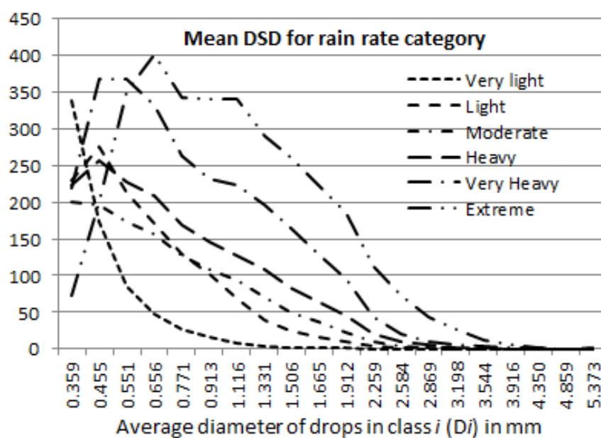
Figure 1. Average observed DSDs for the database for six rainfall rate categories.
